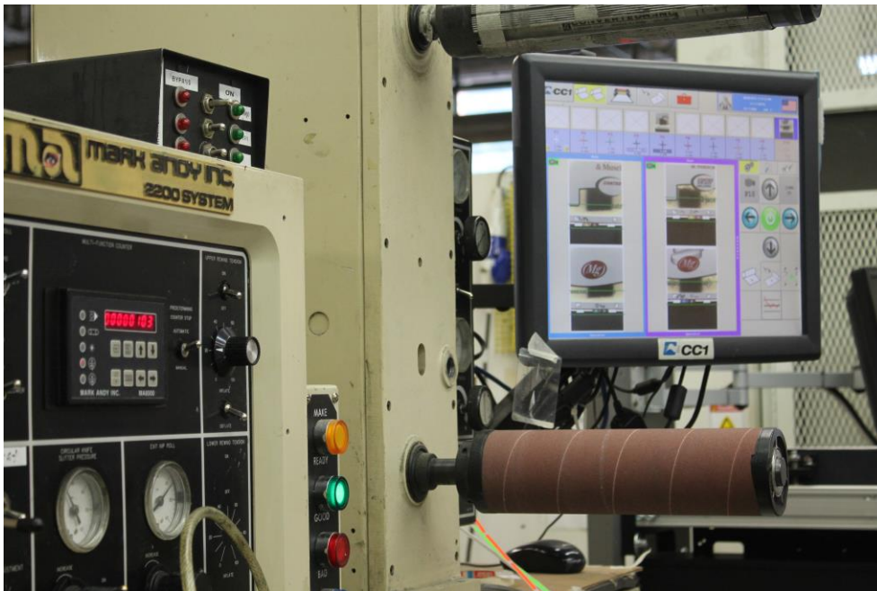
CC1's Camera-based Automatic Register Controls help address the need in today's label printing market for greater and tighter register accuracy, while helping lower production costs
